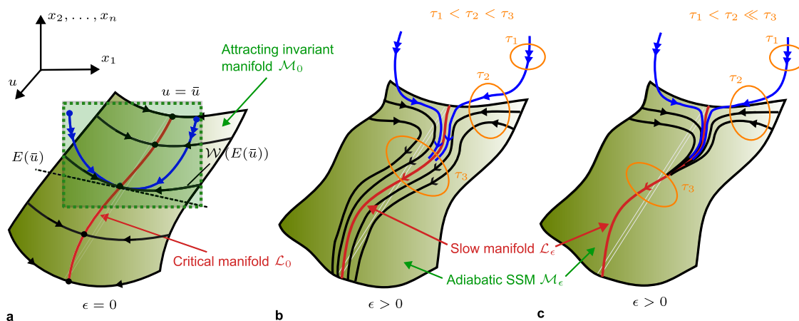
Fig. 2 | Adiabatic spectral submanifolds and slow-manifold reduction across time scales. a Geometry of the attracting invariant manifold \mathcal{M}_0 formed by a family of SSMs, \mathcal{W}(E(u)) , parametrized by the external forcing parameter u , for \epsilon = 0 . For simplicity, u is assumed to be a scalar in this plot. The critical manifold \mathcal{L}_0 consists of the collection of the fixed points corresponding to each value of u . b For \epsilon \neq 0 , the manifold \mathcal{M}_0 perturbs into an aSSM, \mathcal{M}_\epsilon , and \mathcal{L}_0 perturbs into a slow manifold,
