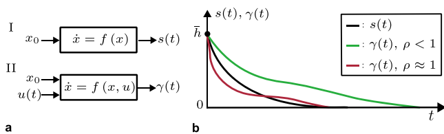
Fig. 3 | Slowness measure compares controlled and autonomous transient dynamics. a Autonomous system (I) and externally forced system (II). b Comparison of trajectories decaying to zero from the same initial point \bar{h} through autonomous transient decay and under slower ( \rho < 1 ) and faster ( \rho \approx 1 ) control in a regulation task.
