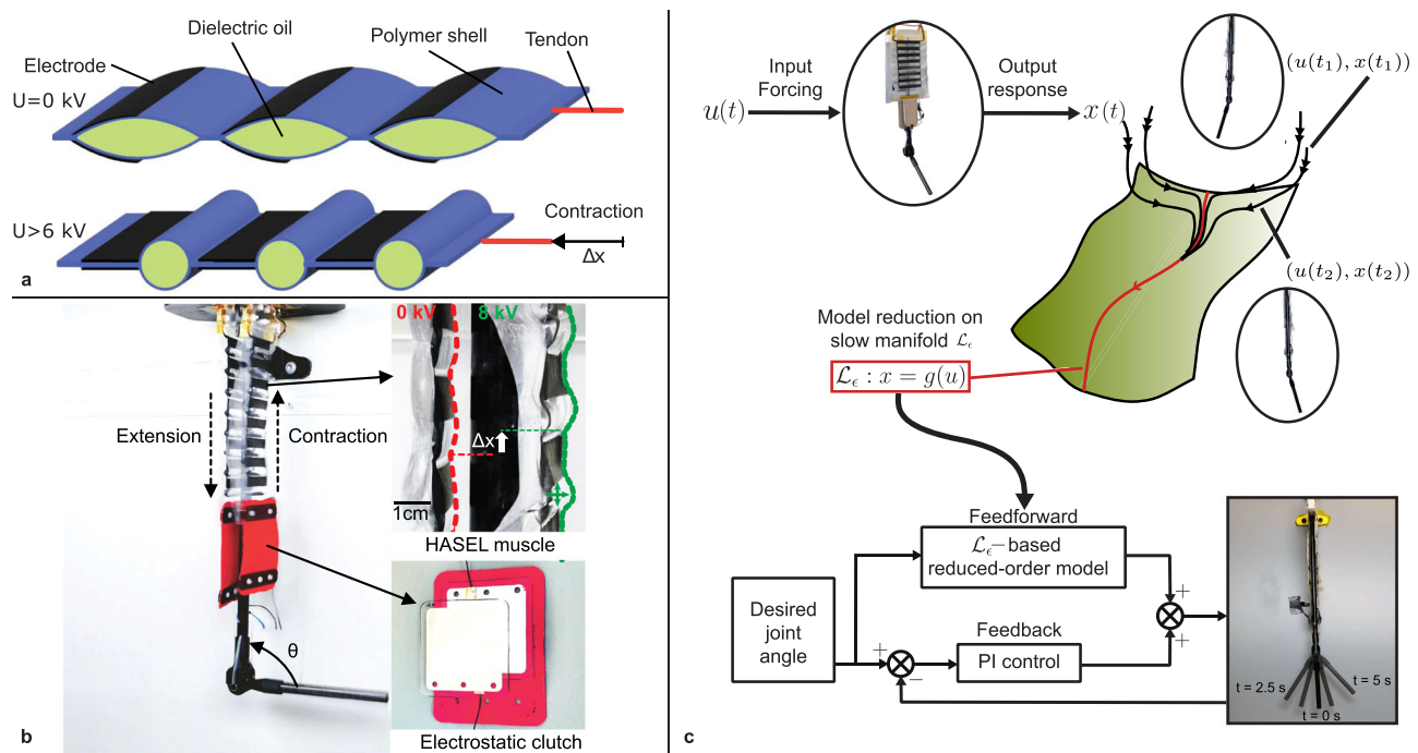
Fig. 1 | Overview of data-driven slow manifold modeling and control for antagonistic artificial muscles. a HASEL actuator working principle: a flexible polymer shell filled with dielectric oil and covered by electrodes; applying voltage (up to U = 8 kV) generates electrostatic pressure that redistributes the fluid, producing axial contraction \Delta x against a tendon load. b Experimental platform: antagonistic musculoskeletal joint actuated by HASEL artificial muscles paired with electrostatic clutches, enabling bidirectional motion and variable stiffness; \theta denotes the joint angle. The inset shows the contraction \Delta x at 0 kV and 8 kV.
