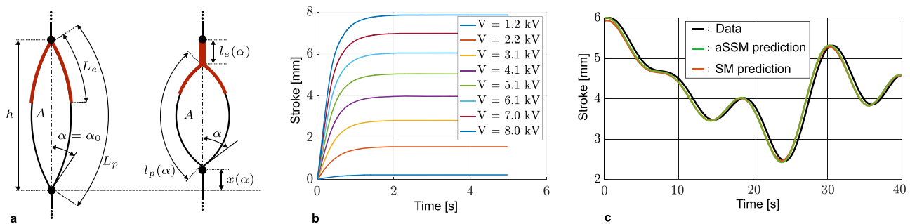
Fig. 5 | Analytical HASEL actuator model and data-driven predictions.
