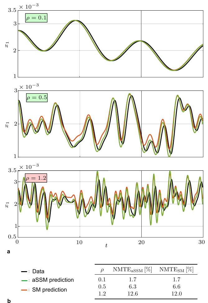
Fig. 4 | Model accuracy depends on the external forcing rate. a Comparison between the aSSM-based and the SM-based reduced-order model of the SDOF of Eq. (10) under random external excitations with increasing speed ( \rho = 0.1 (top), \rho = 0.5 (middle) and \rho = 1.2 (bottom)). As predicted by theory, the slow manifold approximation is accurate when \rho \ll 1 , while in the last case, even the leading-order aSSM-based approximation breaks down. b Legend and table reporting the Normalized Mean Trajectory Error (NMTE) values for the different cases.
