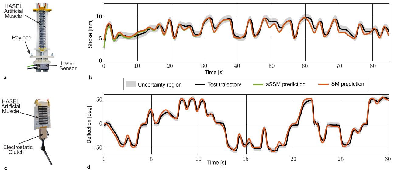
Fig. 6 | Experimental HASEL artificial muscles and data-driven slow manifold predictions. a Single HASEL actuator with payload and laser displacement sensor. b Predictions of the actuator stroke under random forcing: the aSSM-based prediction (green) quickly converges to the SM-based prediction (orange), both closely matching the test trajectory (black); the shaded region indicates the uncertainty region estimated from repeated HASEL actuator characterization trials.
