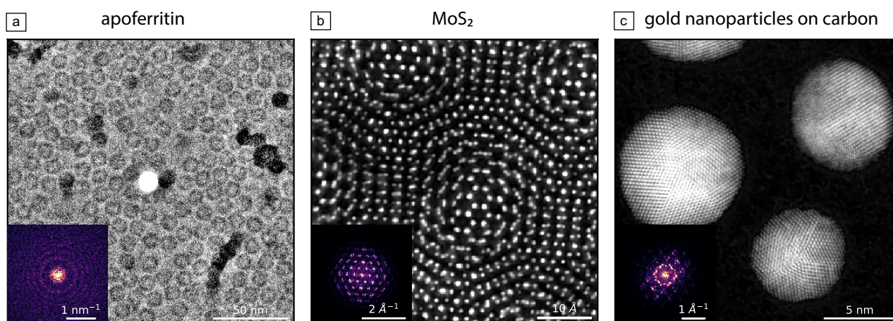
Figure 7. Iterative ptychography reconstructions of (a) apoferritin, 9 (b) MoS 2 , 26 and (c) gold nanoparticles on amorphous carbon. Aberrations coefficients were initialized using direct ptychography reconstructions in Figures 5 and 6.
