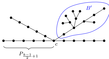
Figure 5. A tree containing three longest paths that avoid B' (so \pi_B = 3 ), and three longest paths that use B' consisting of a P_{(k+1)/2} outside B' and a P_{(k-1)/2} inside (so \tau_B = 3 ).
